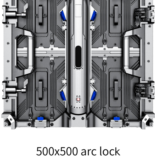
500x500 arc lock
